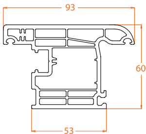
603.5 Outward Window Sash 5 Chamber
