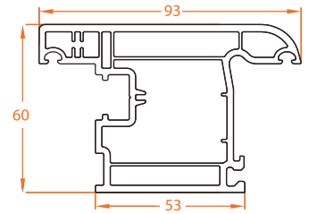
603.3 Outward Window Sash 3 Chamber
