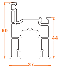
802.4 60mm Window Sash
