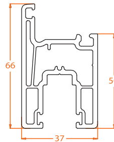
802.2 66mm Window Sash
