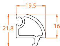
805.1 Beading 5mm Round
