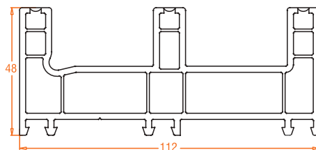
8801.5 Sliding frame 112mm
