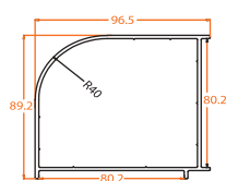
809.4 80-Curved Corner
