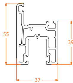
802.1 55mm Window Sash
