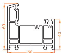
601.1 Frame 60mm Opal
