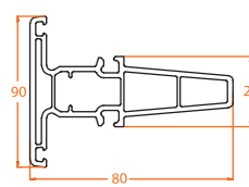
804.2 Frame Mullion
