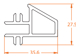
109.3 Frame Connector
