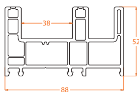
8801.1 Sliding Frame 88mm
