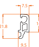
805.4 Beading 16mm
