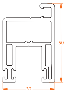
8806.2 50mm Screen Sash
