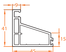
606.1 Openable Screen Sash
