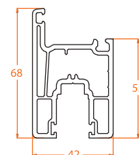
8802.2 68mm Window Sash
