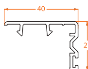
809.1 Small Interlock
