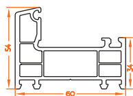
601.5 Small Openable Frame
