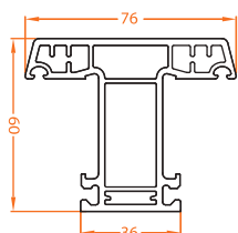
604.1 Mullion 60mm Opal
