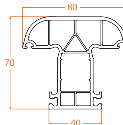
604.5 70/60 Mullion
