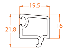
805.12 Beading 5mm choras
