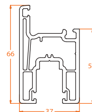
802.2 66mm Window Sash
