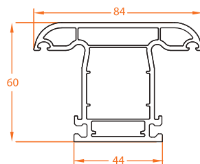
604.3 Mullion 60mm Royal
