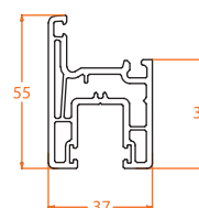
802.1 55mm Window Sash
