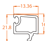
805.3 Beading 12mm
