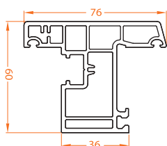
603.1 Outward Window Sash
