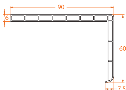
109.8 Border Profile
