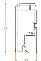
806.2 66mm Screen Sash
