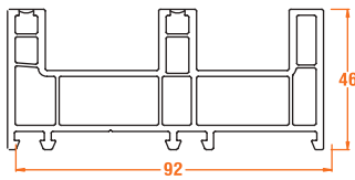
801.4 Sliding Frame 92mm
