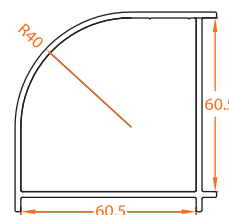
609.4 60-60 Curved Corner
