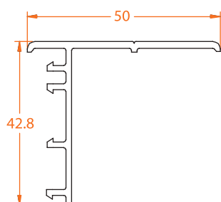
109.7 Small Border Profile
