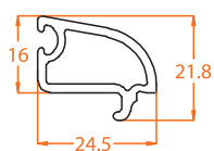
8805.1 5mm Glass Beading
