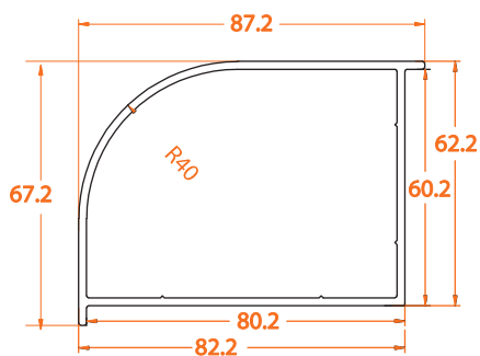
109.4 80-60 Curved Corner
