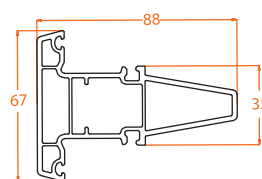
8804.2 Fixed Frame Mullion
