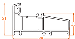
8801.3 Fixed Frame
