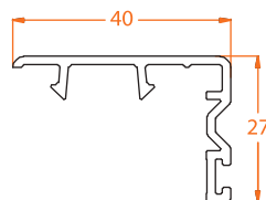
809.1 Small Interlock
