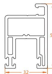
8806.2 50mm Screen Sash
