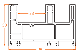
801.1 Sliding Frame 80mm
