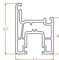
8802.1 57mm Sash
