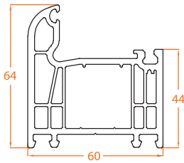
601.3 Frame 5 Chamber Royal
