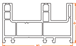
801.3 Sliding Frame 80mm
