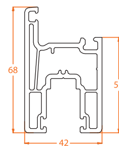
8802.2 68mm Window Sash
