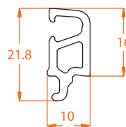
8805.4 20mm Glass Beading
