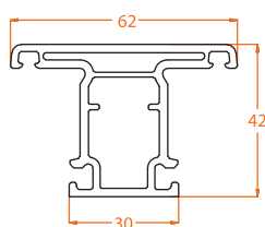
8804.1 Sash Mullion
