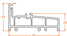
801.2 Sliding Fixed Frame
