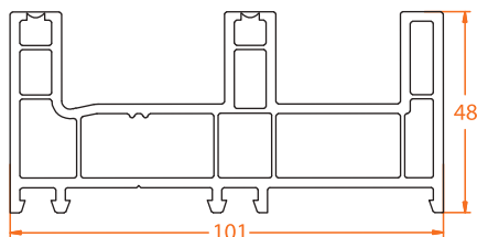
8801.4 Sliding Frame 101mm
