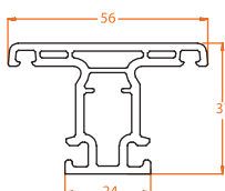
804.1 Sash Mullion
