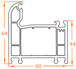
601.2 Frame 60mm Royal
