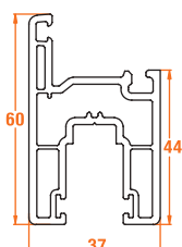
802.4 60mm Window Sash
