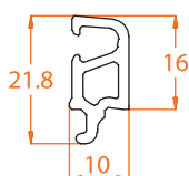
8805.4 20mm Glass Beading
