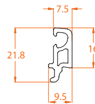
805.4 Beading 16mm
